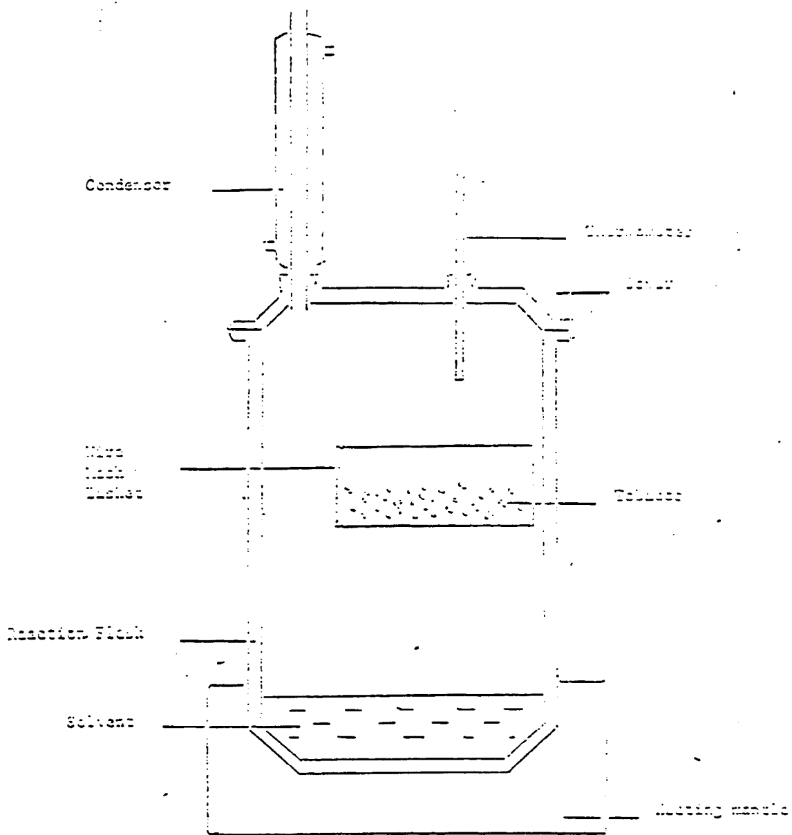
Schematic Diagram of Apparatus (Laboratory)
